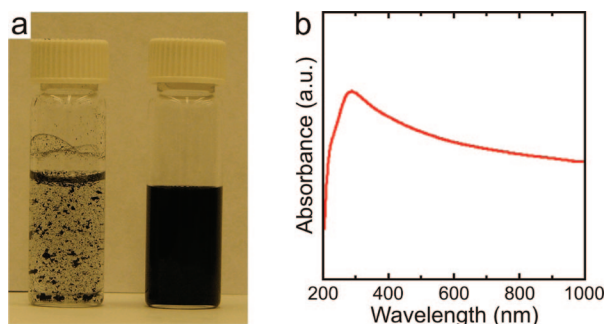
Figure 1. (a) A photograph of FGSs (left) and SDS-FGS aqueous dispersion (right); (b) UV-vis absorbance of the SDS-FGS aqueous dispersion.
